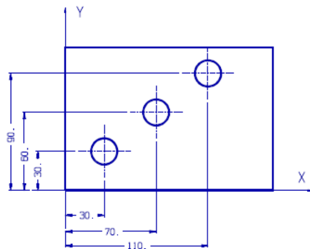
Fig.2-3 Absolute System
