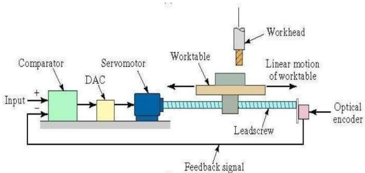
Closed loop Control System
