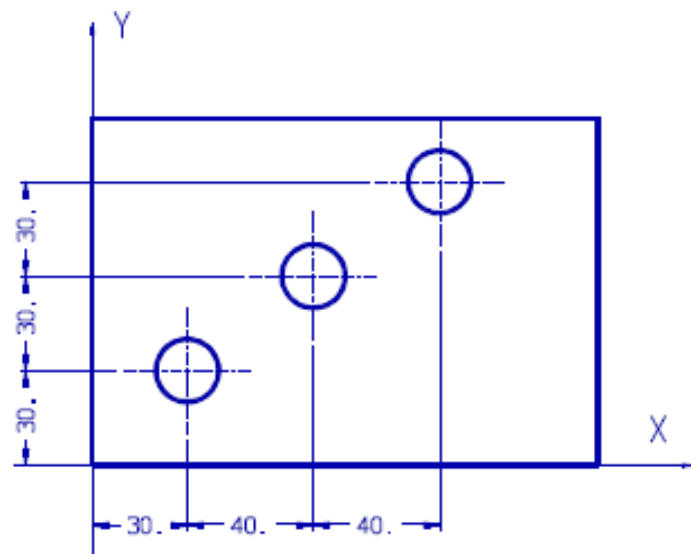
Fig.2-2 Incremental System
